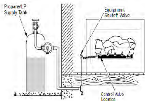
Checking Gas Joints (Natural Gas Only)
